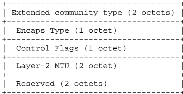
Figure 3: Layer2 Info Extended Community
