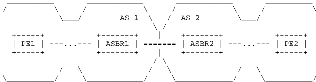
Figure 5: Inter-AS VPLS
