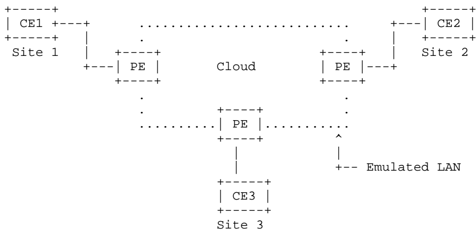
Figure 1: Topological Model of a VPLS for Customer X with three sites
